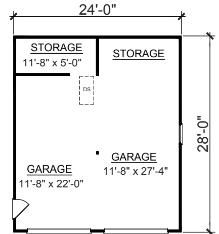
DETACHED GARAGE 672 Sq. Ft.
