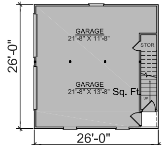
DETACHED GARAGE PLAN
