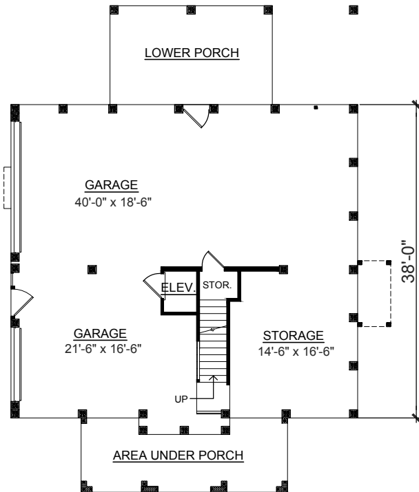
GROUND FLOOR PIER PLAN
